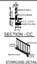
STAIRCASE DETAILS
