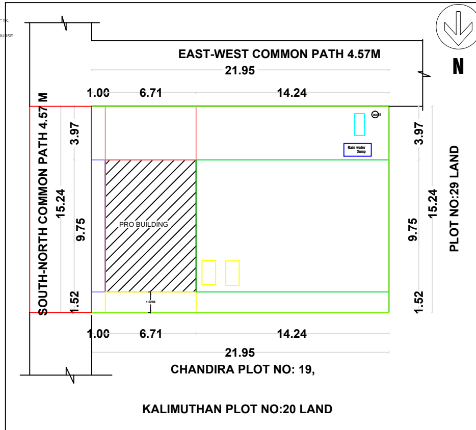
SITE PLAN & KEY PLAN
