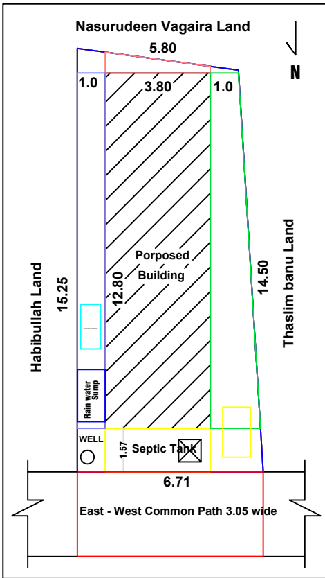
SITE PLAN CUM KEYPLAN
