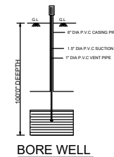
BORE WELL
