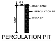
PERCOLATION PIT
