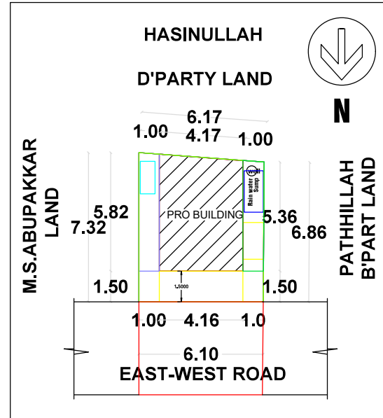
SITE PLAN & KEY PLAN
