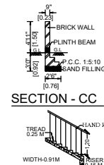
STAIRCASE DETAILS
