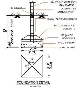
FOUNDATION DETAIL
