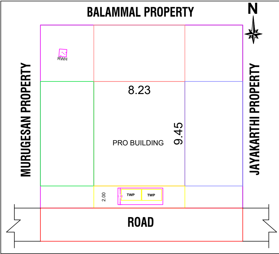
SITE PLAN
