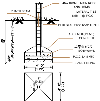
FOUNDATION DETAIL
