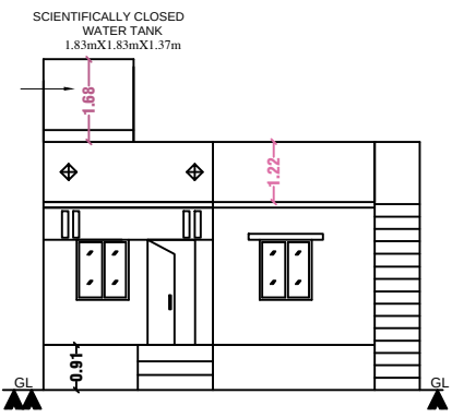
FRONT ELEVATION
