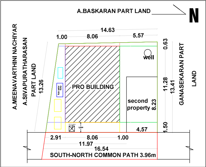
SITE PLAN & KEY PLAN
