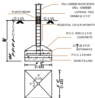
FOUNDATION DETAIL
