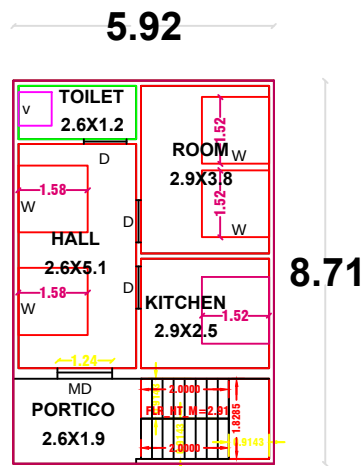
GROUND FLOOR PLAN TERRACE FLOOR PLAN
