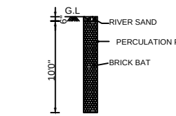
PERCULATION PIT
