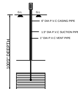
BORE WELL
