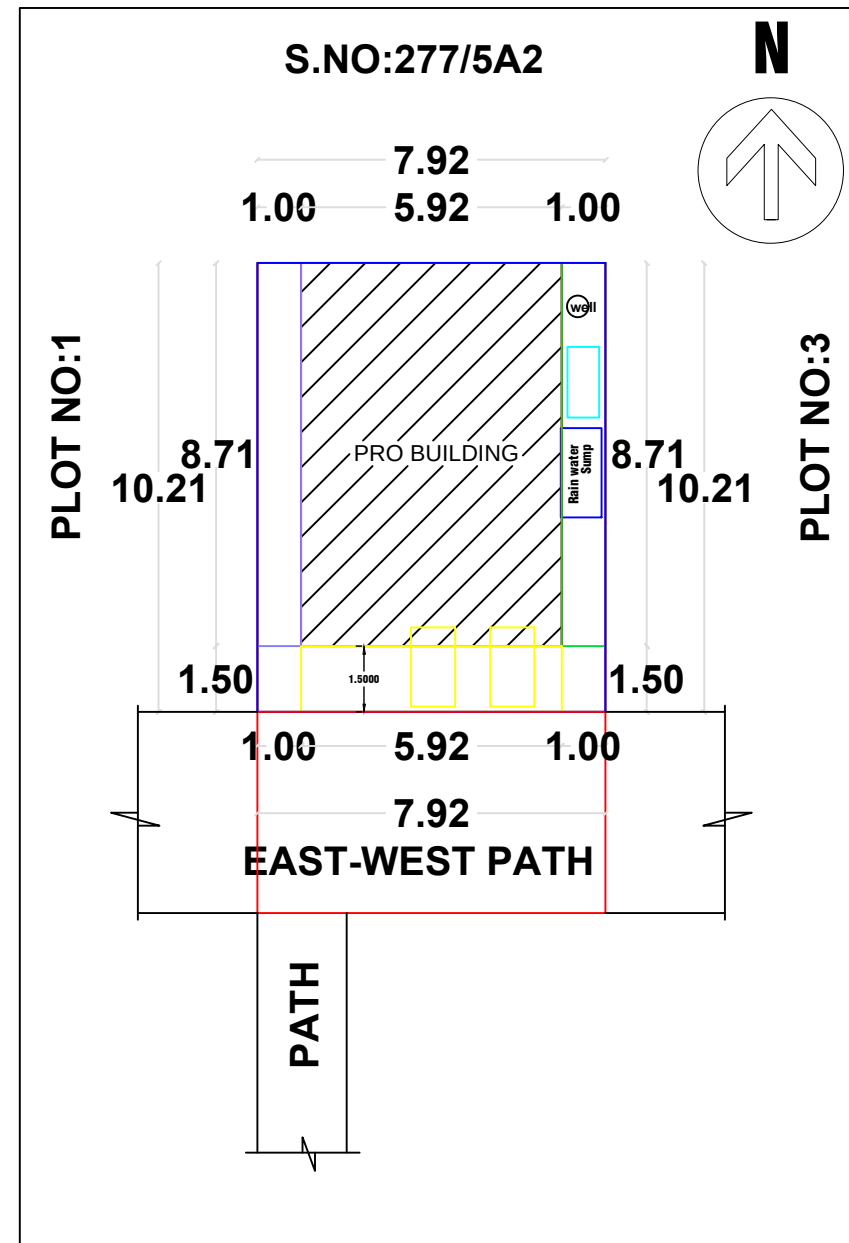
SITE PLAN & KEY PLAN
