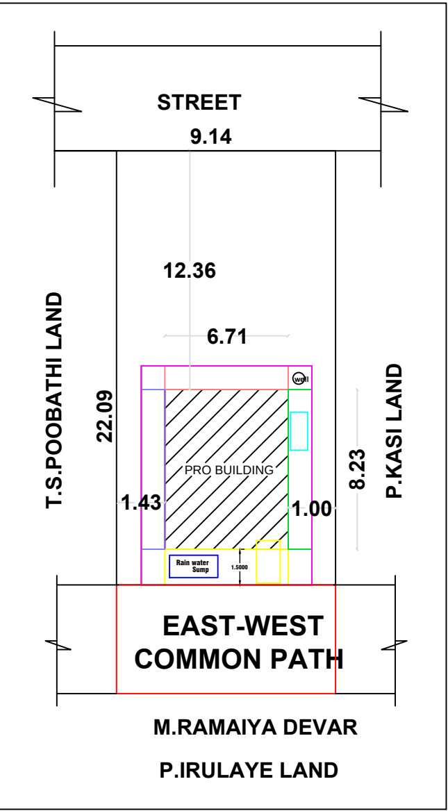
SITE PLAN & KEY PLAN (1:100)
