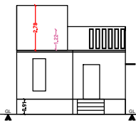
FRONT ELEVATION
