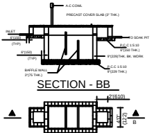
SECTION - BB PLAN OF SEPTIC TANK
