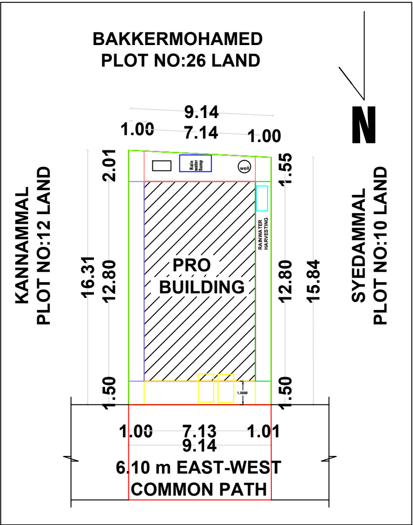
SITE PLAN & KEY PLAN (1:100)
