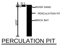
PERCOLATION PIT
