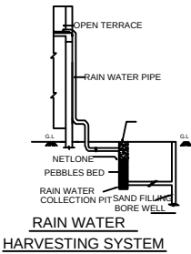
RAIN WATER HARVESTING SYSTEM
