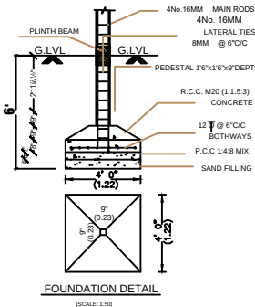
FOUNDATION DETAIL (SCALE: 1:50)
