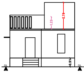
FRONT ELEVATION
