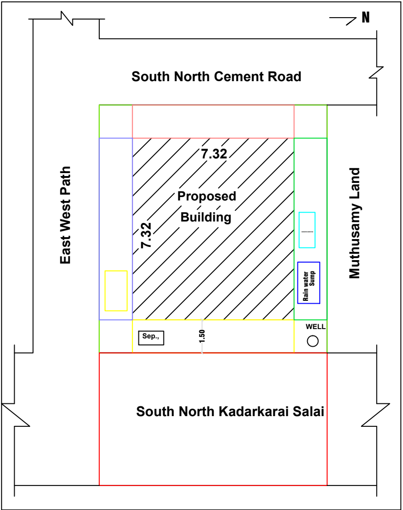
SITE PLAN CUM KEYPLAN
