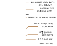
FOUNDATION DETAIL
