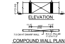
COMPOUND WALL PLAN
