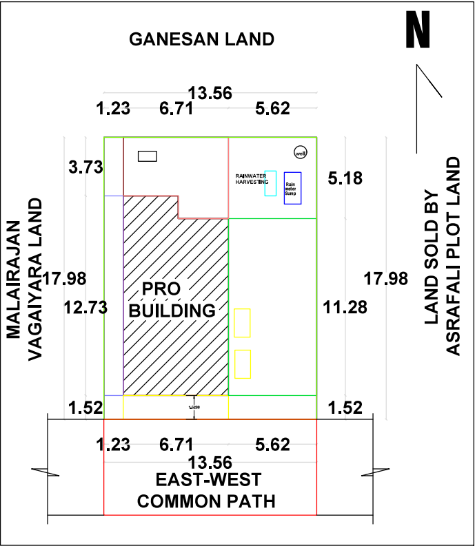
SITE PLAN & KEY PLAN (1:100)
