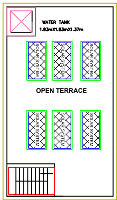
TERRACE FLOOR PLAN
