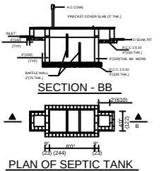
SECTION - BB PLAN OF SEPTIC TANK
