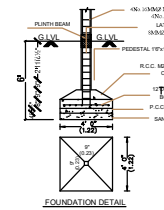
FOUNDATION DETAIL
