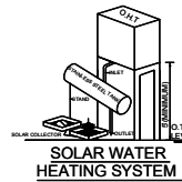
SOLAR WATER HEATING SYSTEM
