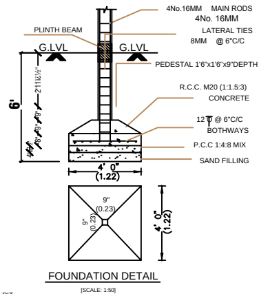
FOUNDATION DETAIL
