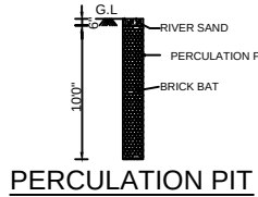
PERCOLATION PIT
