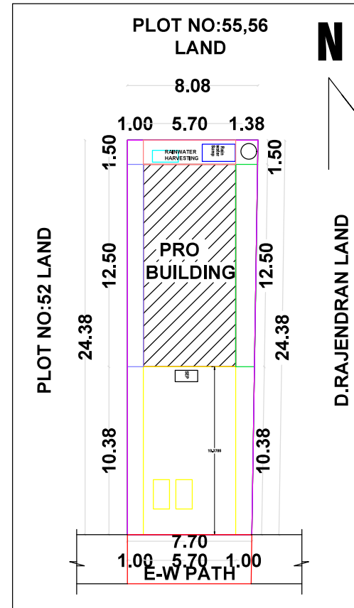
SITE PLAN & KEY PLAN (1:100)
