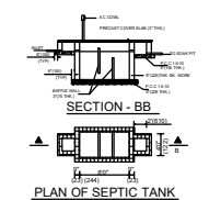
PLAN OF SEPTIC TANK
