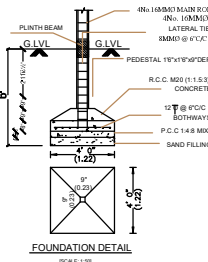
FOUNDATION DETAIL
