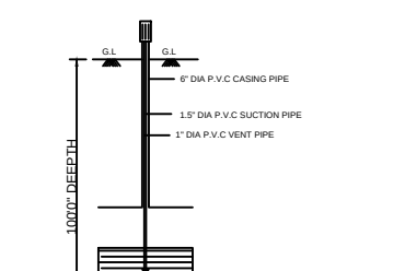
BORE WELL
