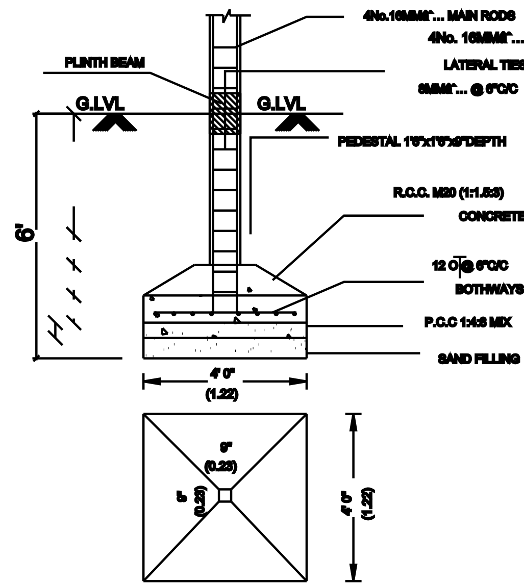
FOUNDATION DETAIL
