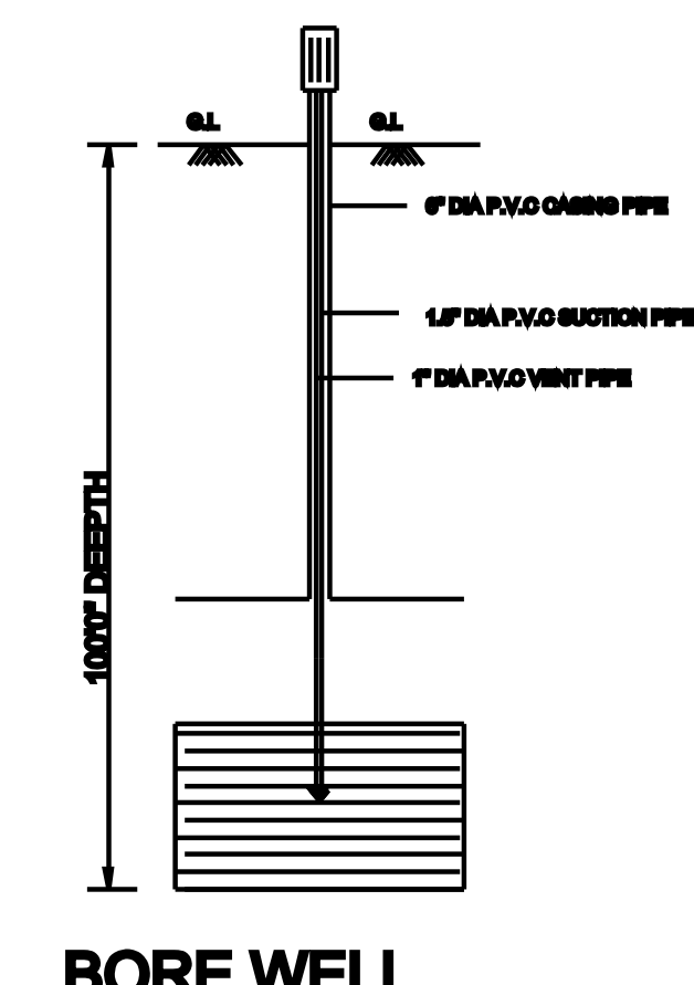
BORE WELL
