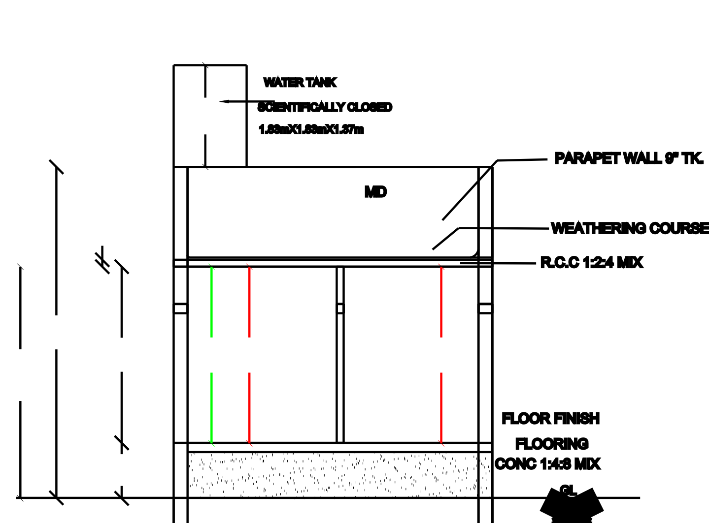
SECTION :A-A'
