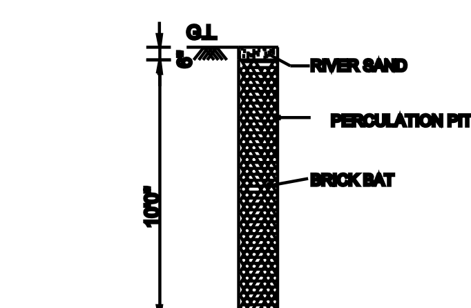
PERCOLATION PIT
