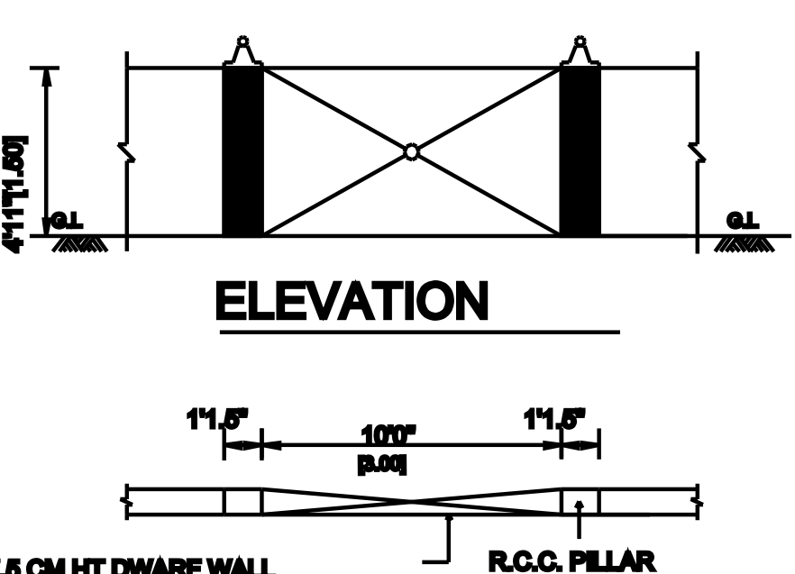
COMPOUND WALL PLAN
