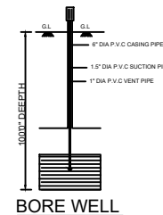
BORE WELL
