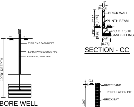
BORE WELL
