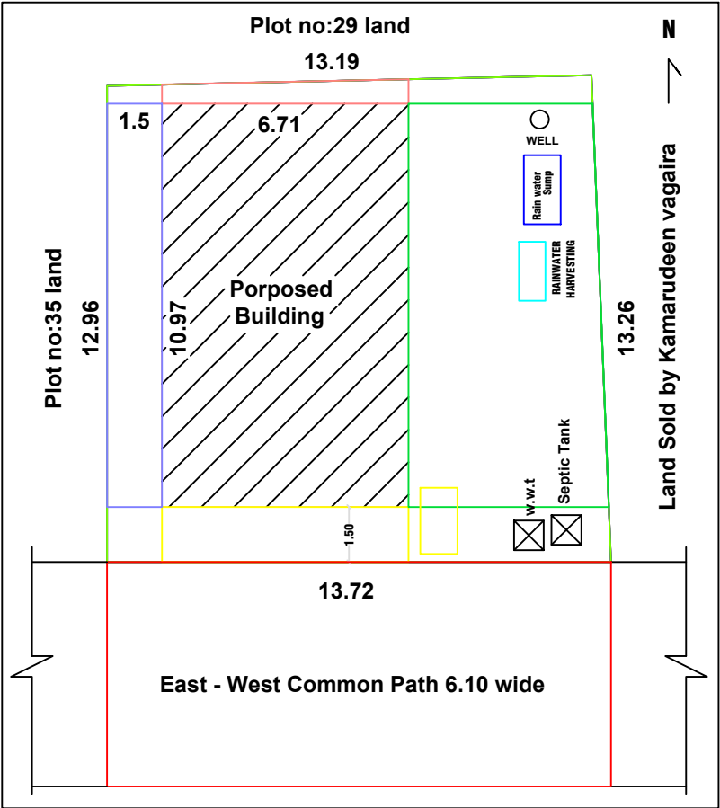
SITE PLAN CUM KEYPLAN
