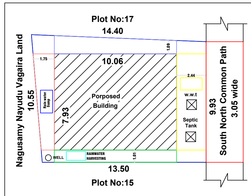
SITE PLAN CUM KEYPLAN
