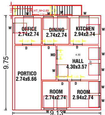
PRO., GROUND FLOOR PLAN
