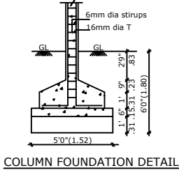
COLUMN FOUNDATION DETAIL
