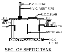
SEC. OF SEPTIC TANK
