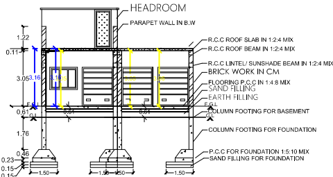
SECTION ON-ON-AA
