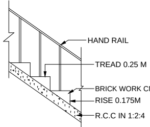
STAIRCASE DETAIL NOT TO SCALE
