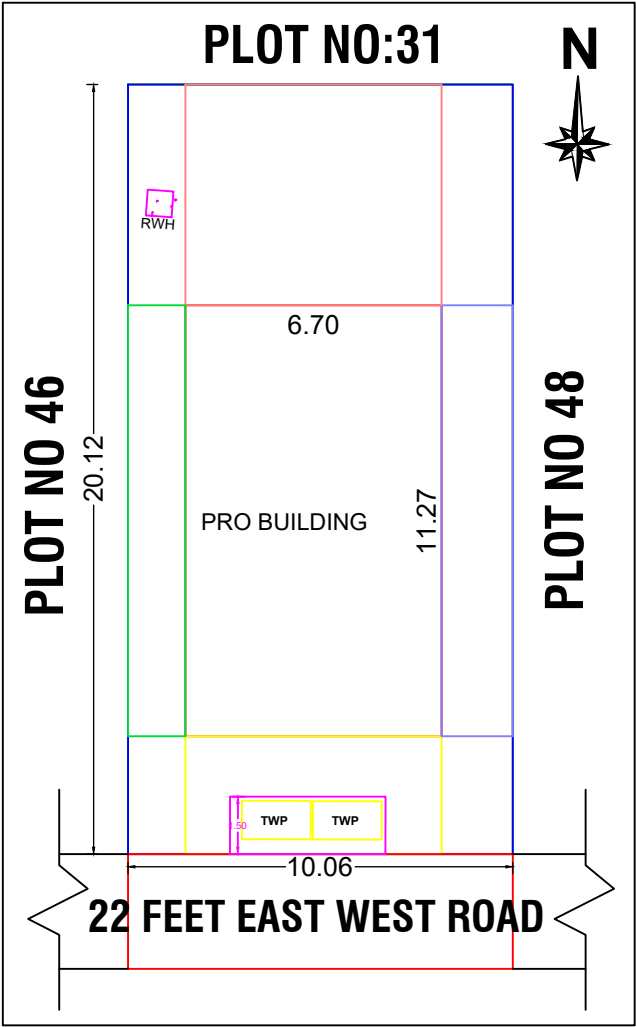
SITE PLAN
