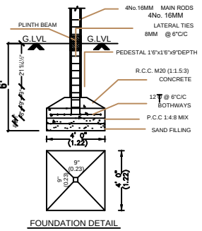
FOUNDATION DETAIL
