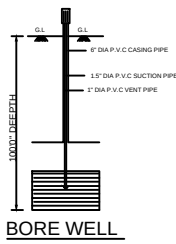
BORE WELL
