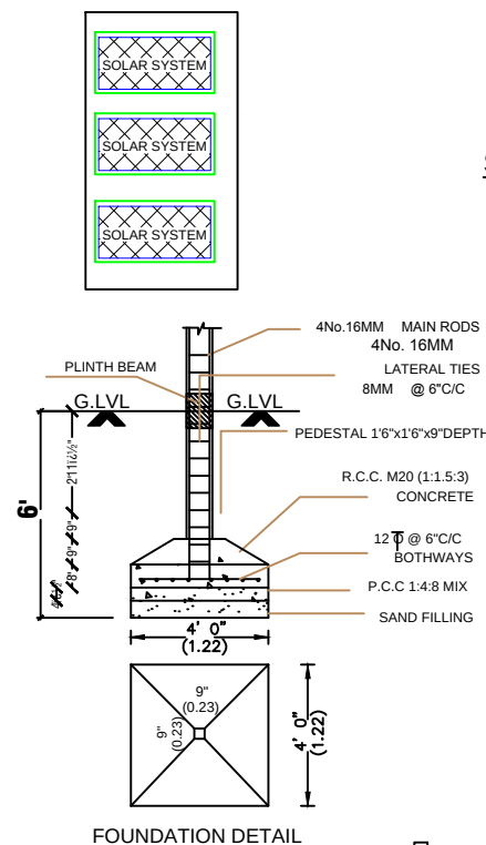
FOUNDATION DETAIL
