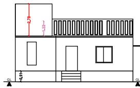
FRONT ELEVATION
