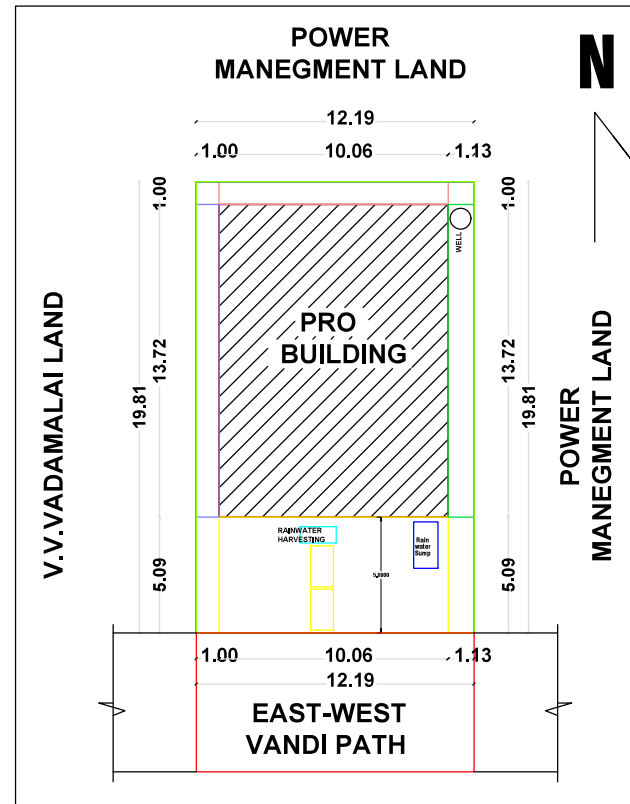
SITE PLAN & KEY PLAN (1:100)
