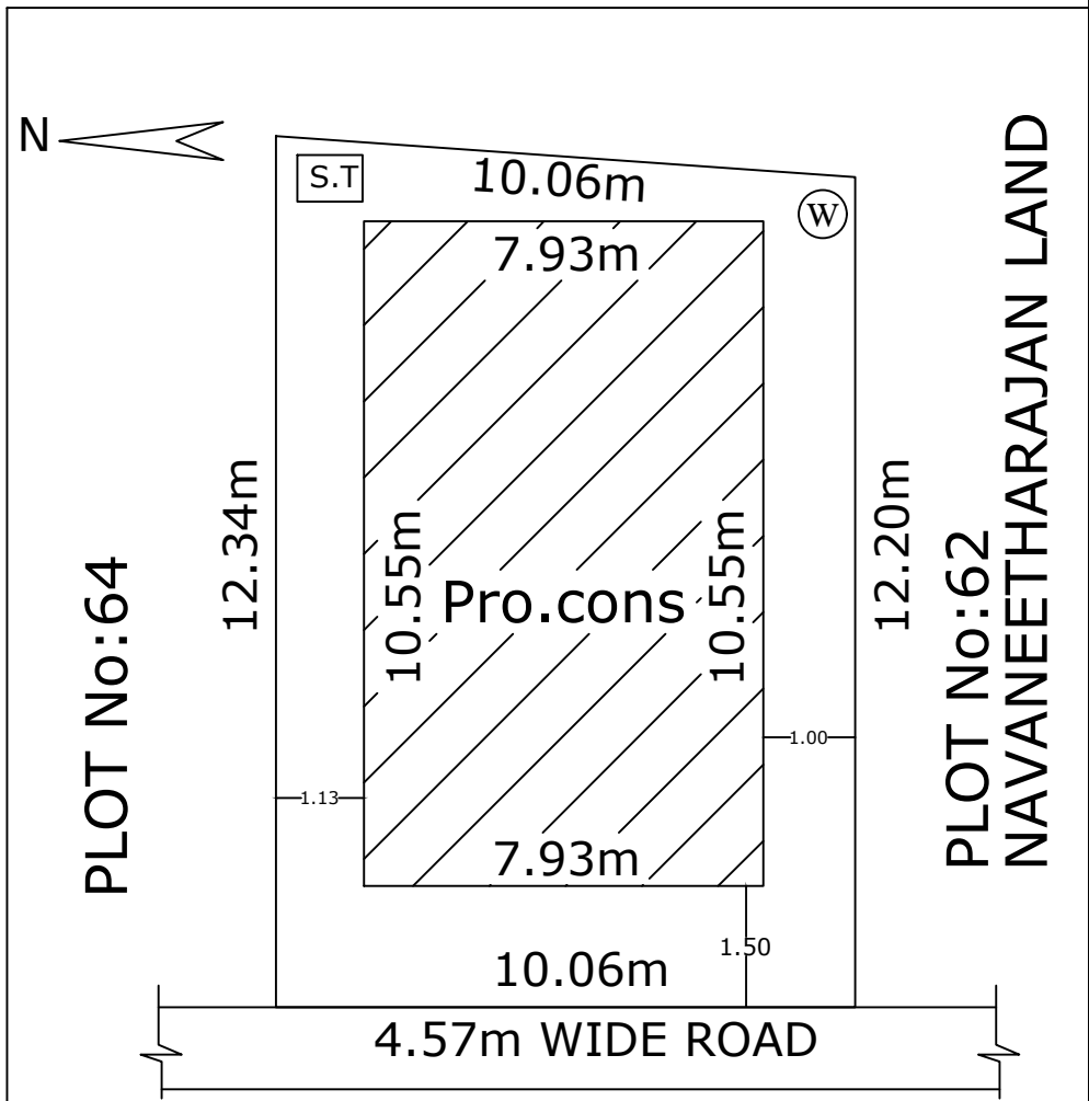
SITE PLAN
