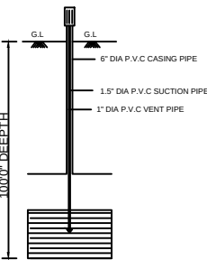
BORE WELL
