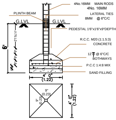
FOUNDATION DETAIL
