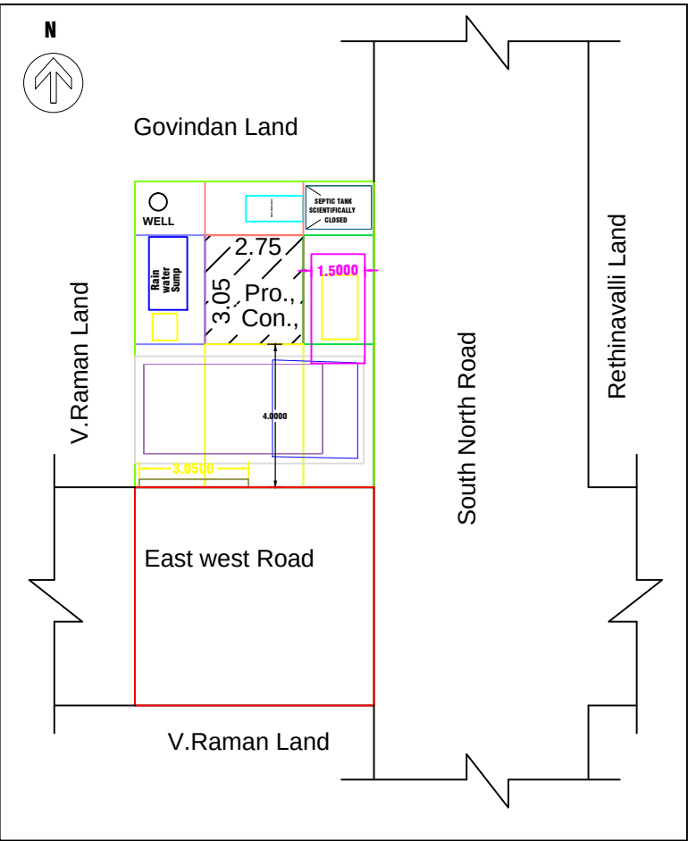
SITE PLAN & KEY PLAN
