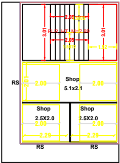
PRO. FIRST FLOOR PLAN
