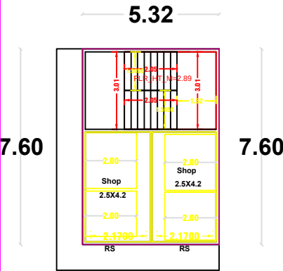
PRO. GROUND FLOOR PLAN
