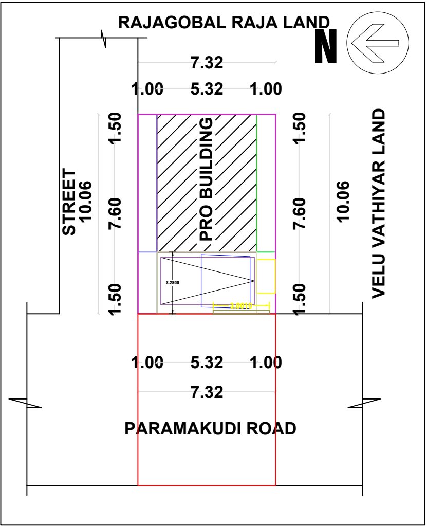
SITE PLAN & KEY PLAN
