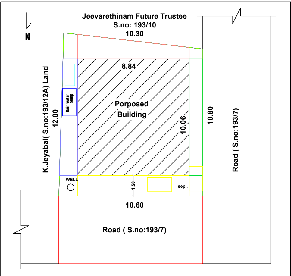
SITE PLAN CUM KEYPLAN
