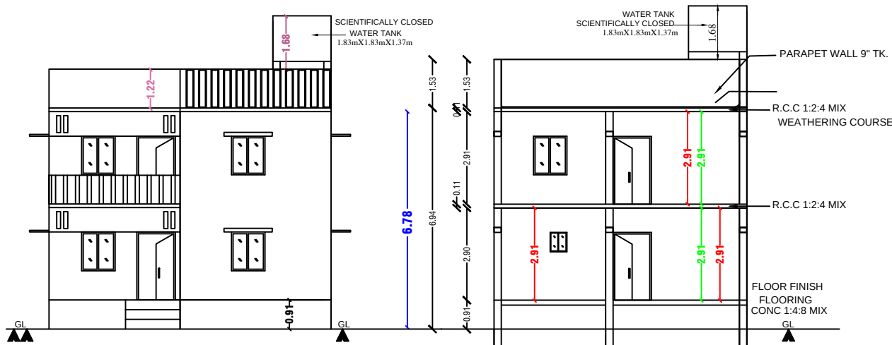
FRONT ELEVATION
