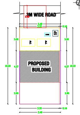
SITE PLAN
