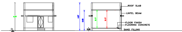
SECTION ON AB
