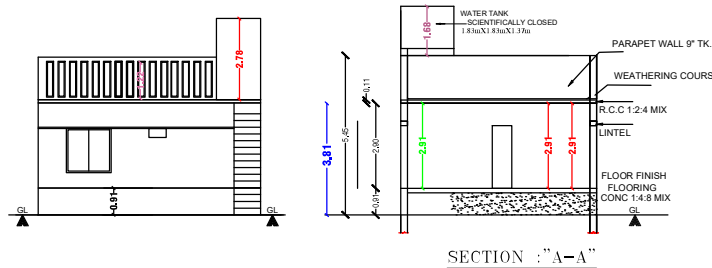
FRONT ELEVATION
