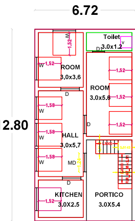
GROUND FLOOR PLAN TERRACE FLOOR PLAN
