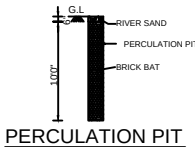
PERCOLATION PIT
