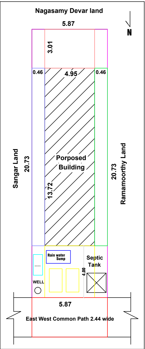
SITE PLAN CUM KEYPLAN
