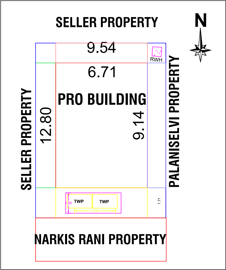
SITE PLAN
