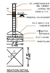
FOUNDATION DETAIL
