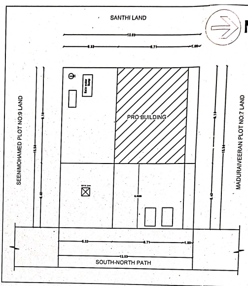
SITE PLAN & KEY PLAN
