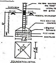
FOUNDATION DETAIL
