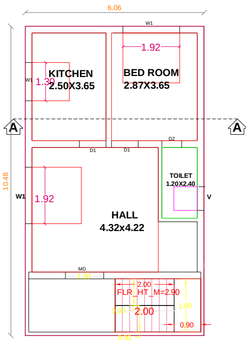
GROUND FLOOR PLAN PROPOSED
