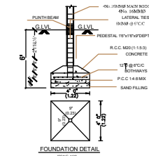
FOUNDATION DETAIL
