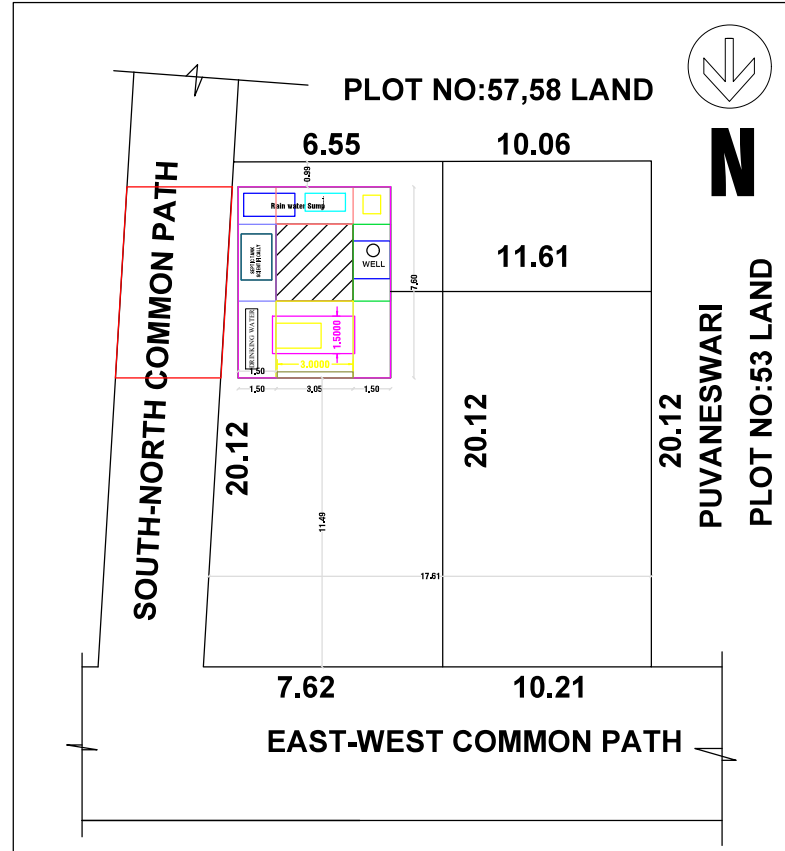
SITE PLAN & KEY PLAN
