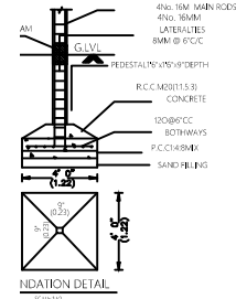
FOUNDATION DETAIL
