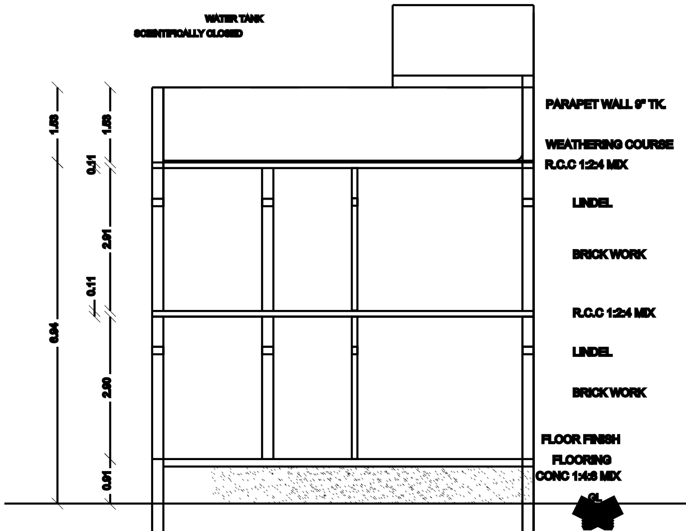
SECTION : "A-A"
