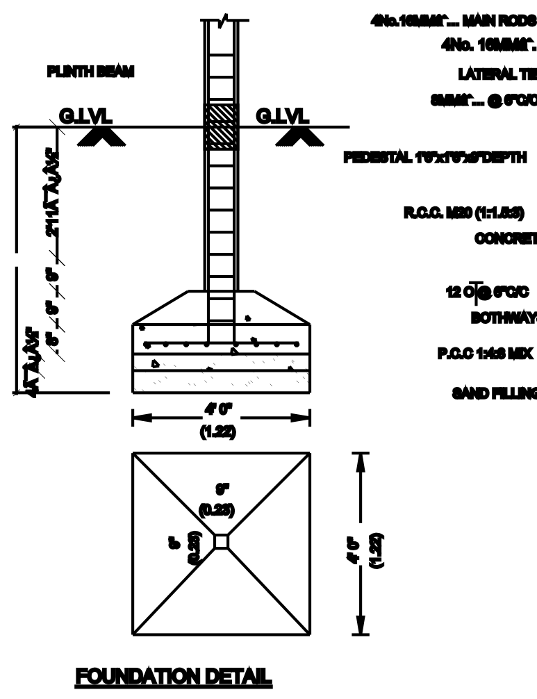
FOUNDATION DETAIL
