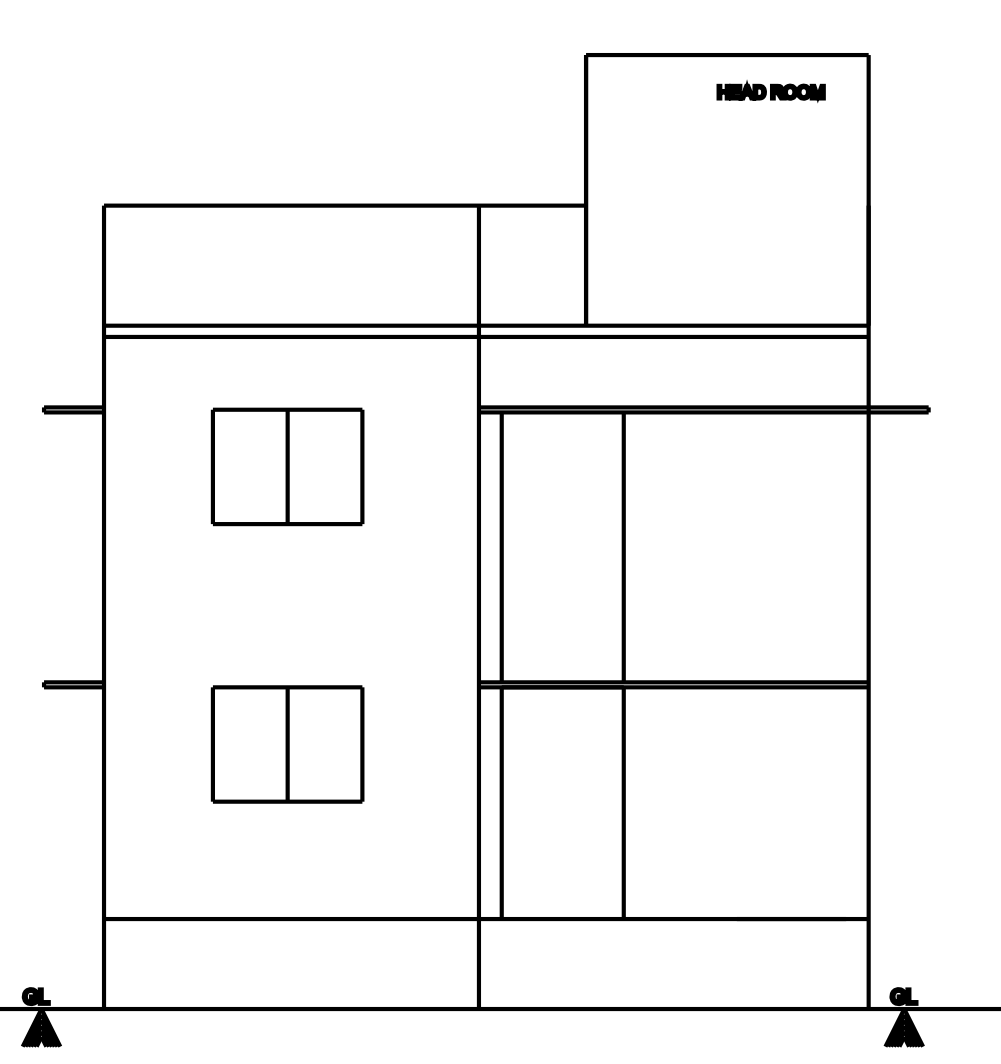
FRONT ELEVATION
