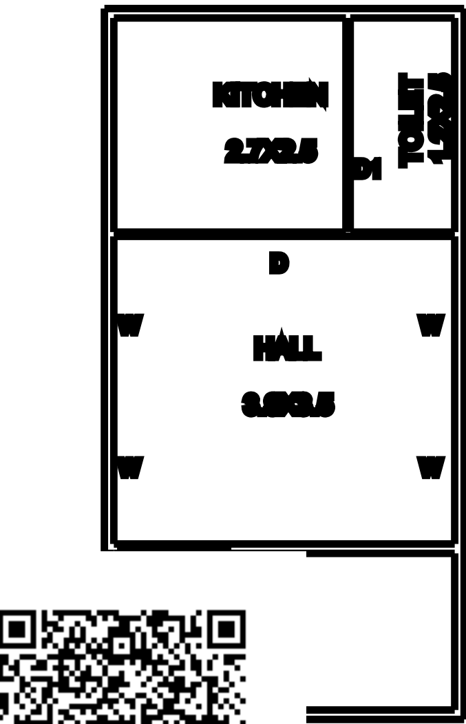
FLOOR PLAN
