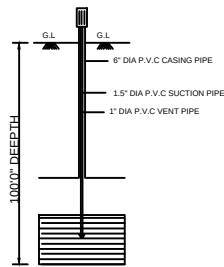
BORE WELL
