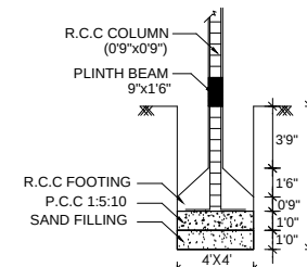
FOUNDATION DETAILS (SCALE 1" = 4'0")
