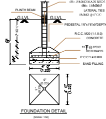
FOUNDATION DETAIL
