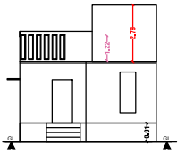
FRONT ELEVATION
