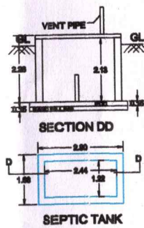
SEPTIC TANK
