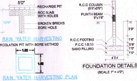
RAIN WATER HARVESTING PLAN
