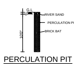
PERCOLATION PIT
