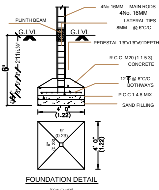
FOUNDATION DETAIL
