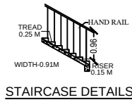
STAIRCASE DETAILS
