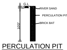
PERCOLATION PIT
